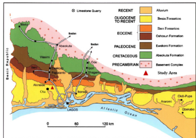
Figure 1. Geological map of the Dahomey (Benin) basin showing the study area 9 .
